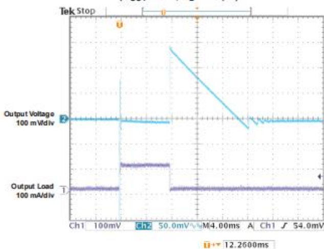
LOAD TRANSIENT RESPONSE VS TIME ( V_{\text{OUT}} = 5\text{ V} , C_L = 10\text{ }\mu\text{F} )
