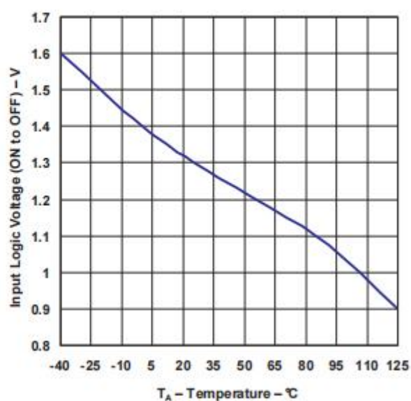
SHUTDOWN THRESHOLD VOLTAGE (ON TO OFF) vs TEMPERATURE
