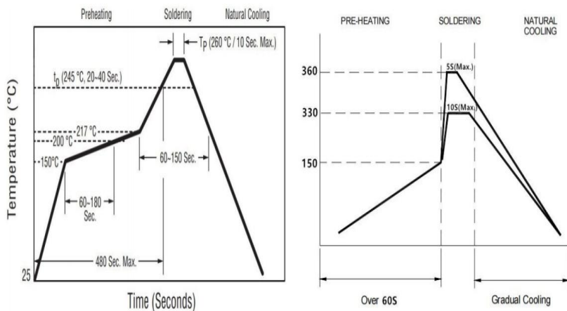
General Reflow Profile & Iron Soldering:
