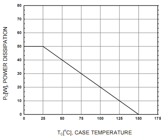
Figure 5. Power Derating
