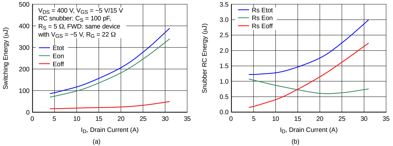
Figure 19. Clamped Inductive Switching Energy (a) and RC Snubber Energy Loss (b) vs. Drain Current at T_J = 25 \text{ }^\circ\text{C} , Turn-On R_{\text{G\_EXT}} = 1 \text{ }\Omega , and Turn-off R_{\text{G\_EXT}} = 22 \text{ }\Omega
