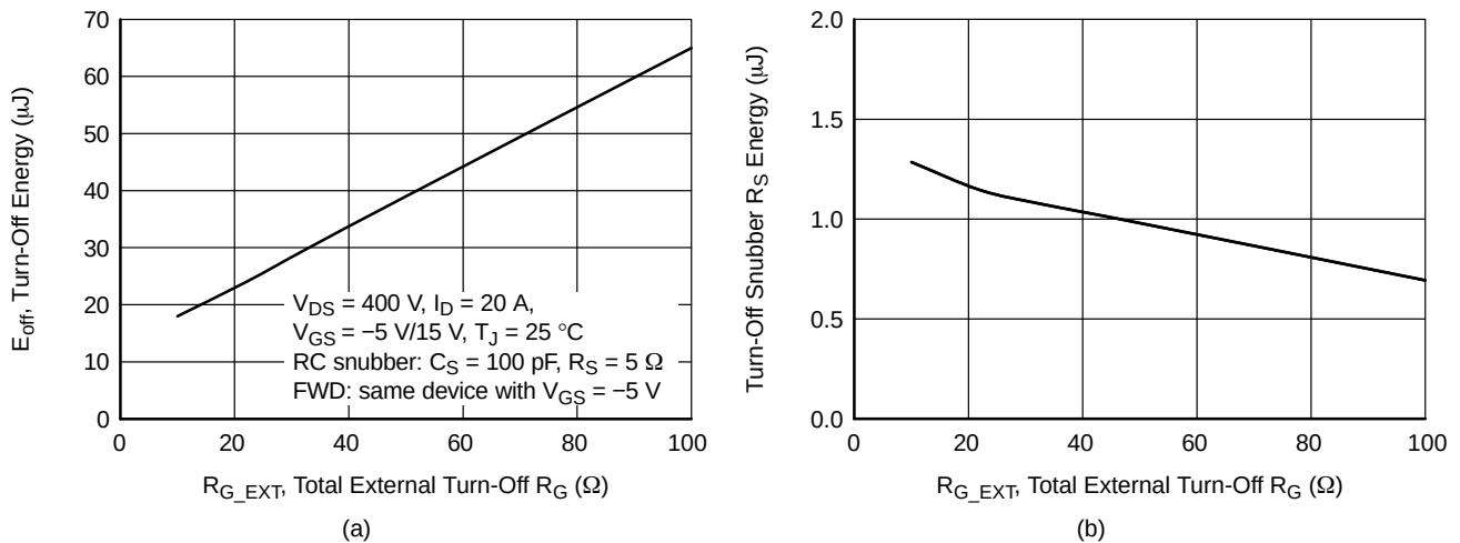
Figure 21. Clamped Inductive Switching Turn-Off Energy Including RC Snubber Energy Loss (a) and RC Snubber Energy Loss (b) as a Function of Total External Turn-Off Gate Resistor R_{\text{G\_EXT}}
