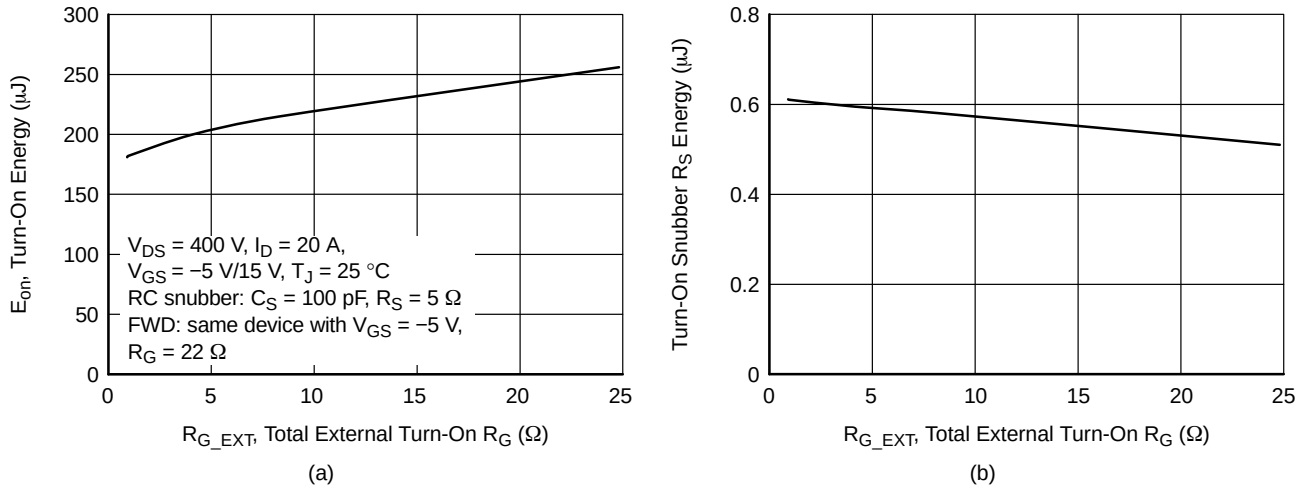
Figure 20. Clamped Inductive Switching Turn-On Energy Including RC Snubber Energy Loss (a) and RC Snubber Energy Loss (b) as a Function of Total External Turn-On Gate Resistor R_{\text{G\_EXT}}
