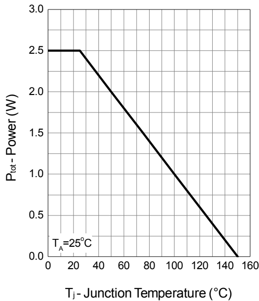
Fig1. Power Dissipation
