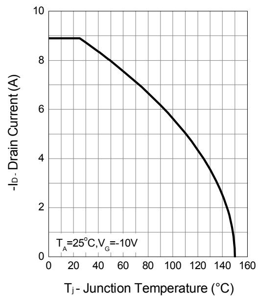
Fig2. Drain Current
