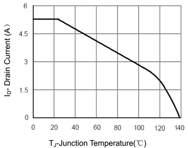
Figure 4 Drain Current
