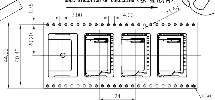
DETAIL 1
