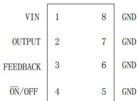
Figure 2.1: SOP8
