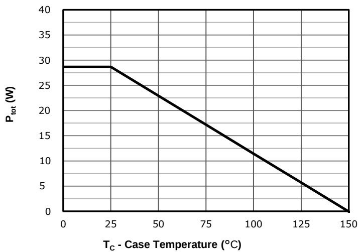
Fig 9: Power Dissipation
