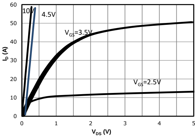
Fig 1: Output Characteristics
