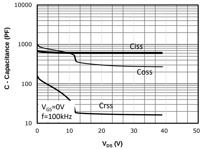
Fig 8: Capacitance Characteristics
