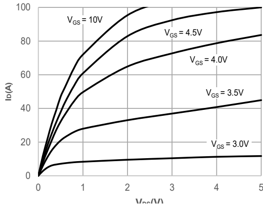
Figure 1: Output Characteristics
