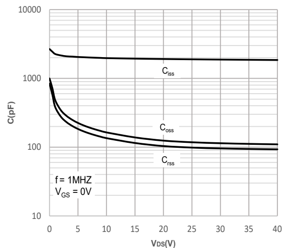
Figure 6: Capacitance Characteristics
