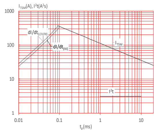
FIG.6: Non-repetitive surge peak on-state current for a sinusoidal pulse with width t_p < 20ms , and corresponding value of I^2t (I - II - III: di/dt < 70A/\mu s ; IV: di/dt < 40A/\mu s )
