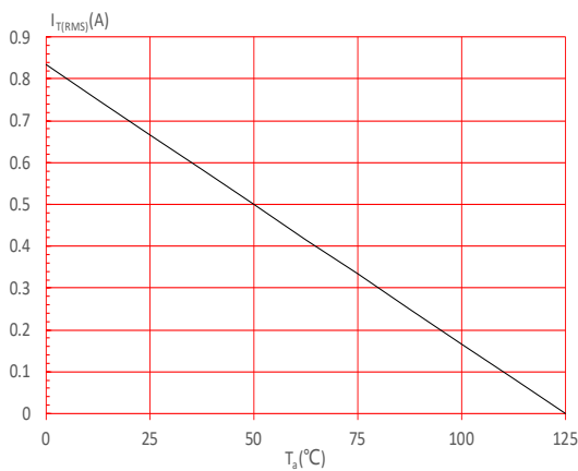
FIG.5: On-state characteristics
