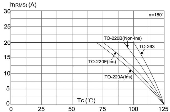
FIG.2: on-state current versus case temperature
