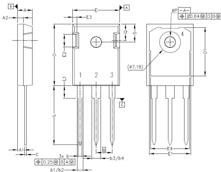
Package TO-247-3
