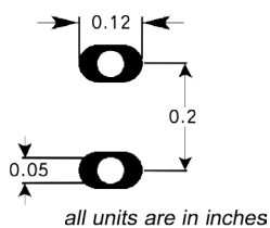
TO-220-2
