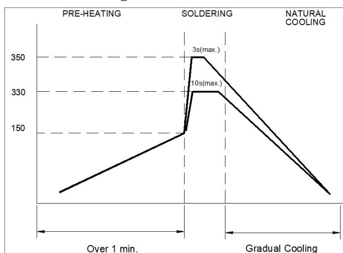
Figure 2. Hand Soldering
