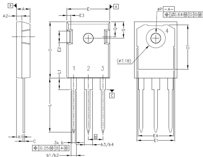
Package TO-247-3
