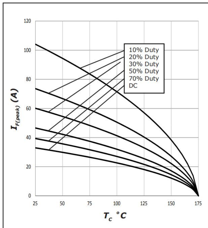
Figure 3. Current Derating
