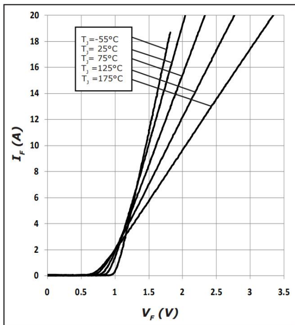
Figure 1. Forward Characteristics
