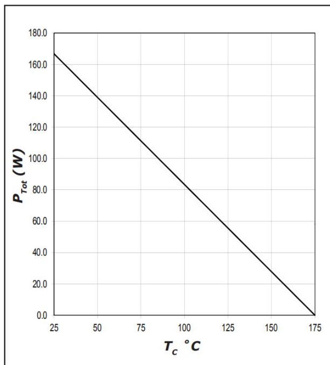
Figure 4. Power Derating
