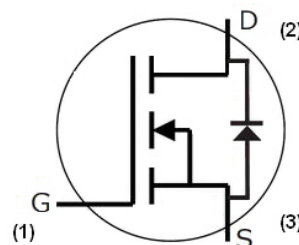
TO-247-3 Package
