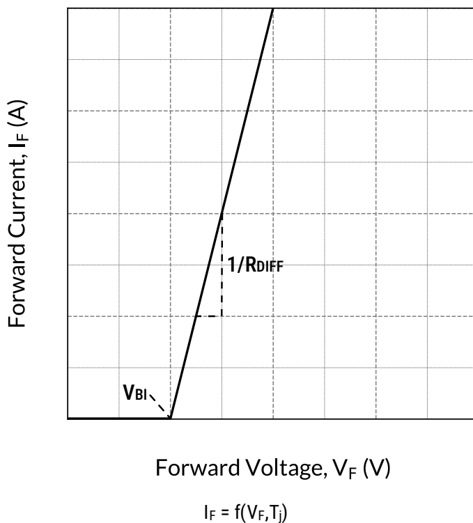
Figure 10: Forward Curve Model (Per Leg)
