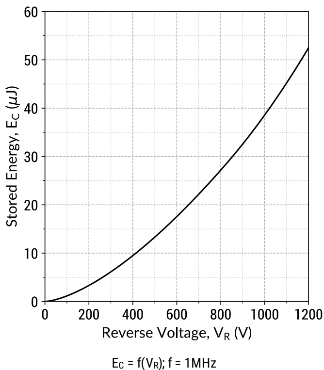
Figure 8: Typical Capacitive Energy vs Reverse Voltage Characteristics (Per Leg)
