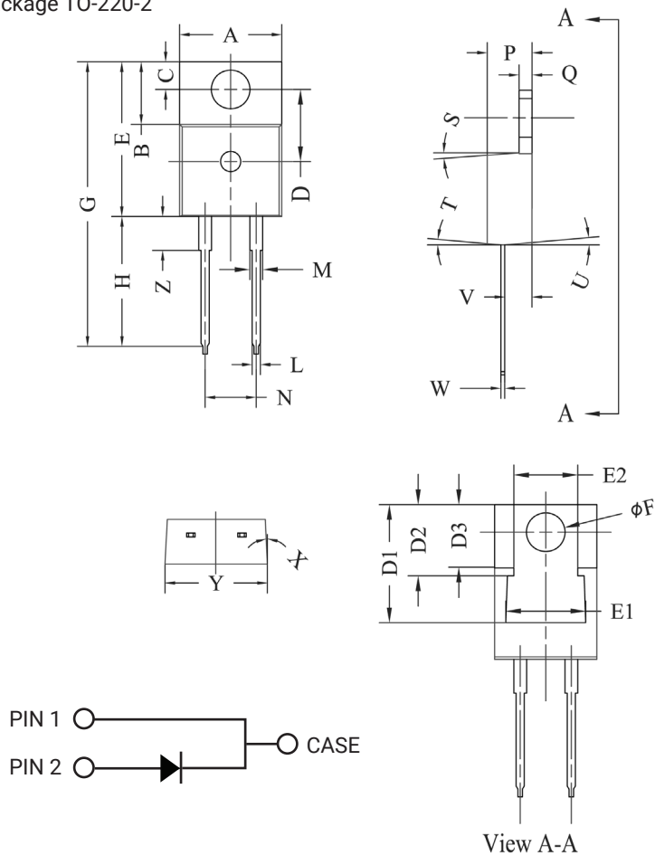
Package TO-220-2
