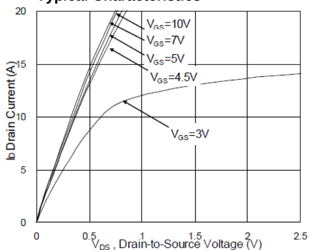
Typical Characteristics
