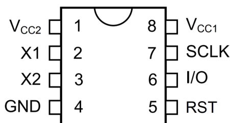
DIP-8/SOP-8/MSOP-8
