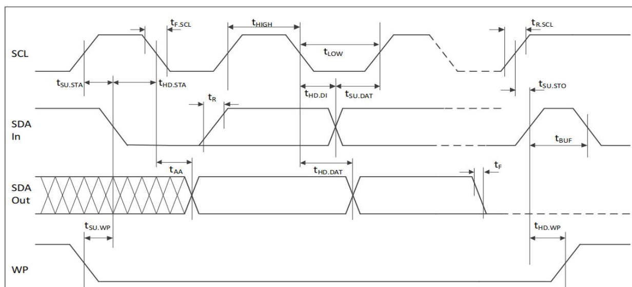
Figure 19 Bus Timing
