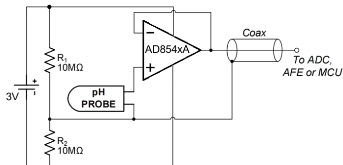
Figure 7. Buffered pH Probe
