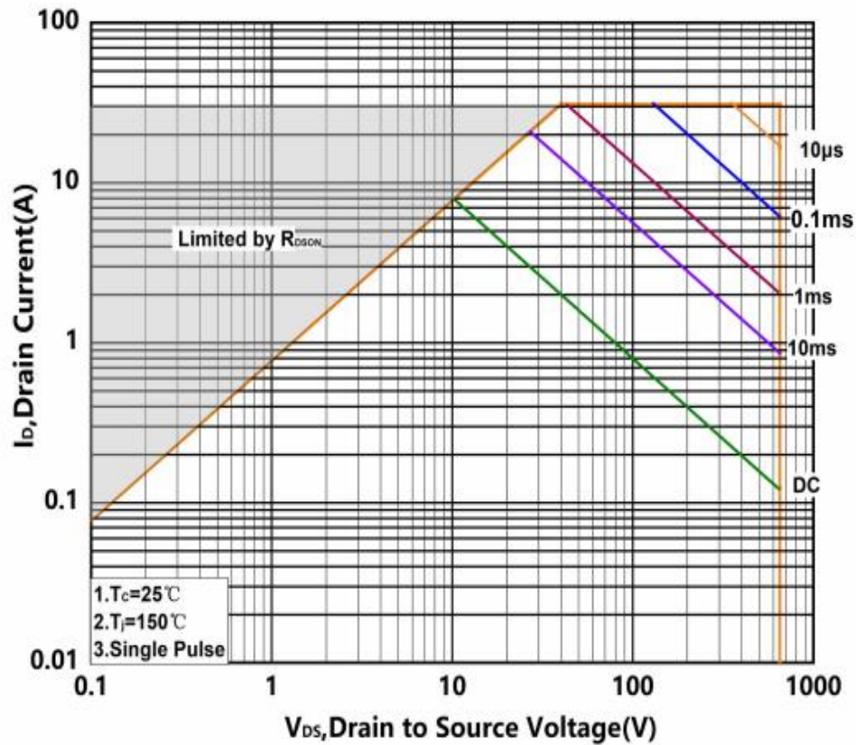
Figure.11 Safe Operating Area
