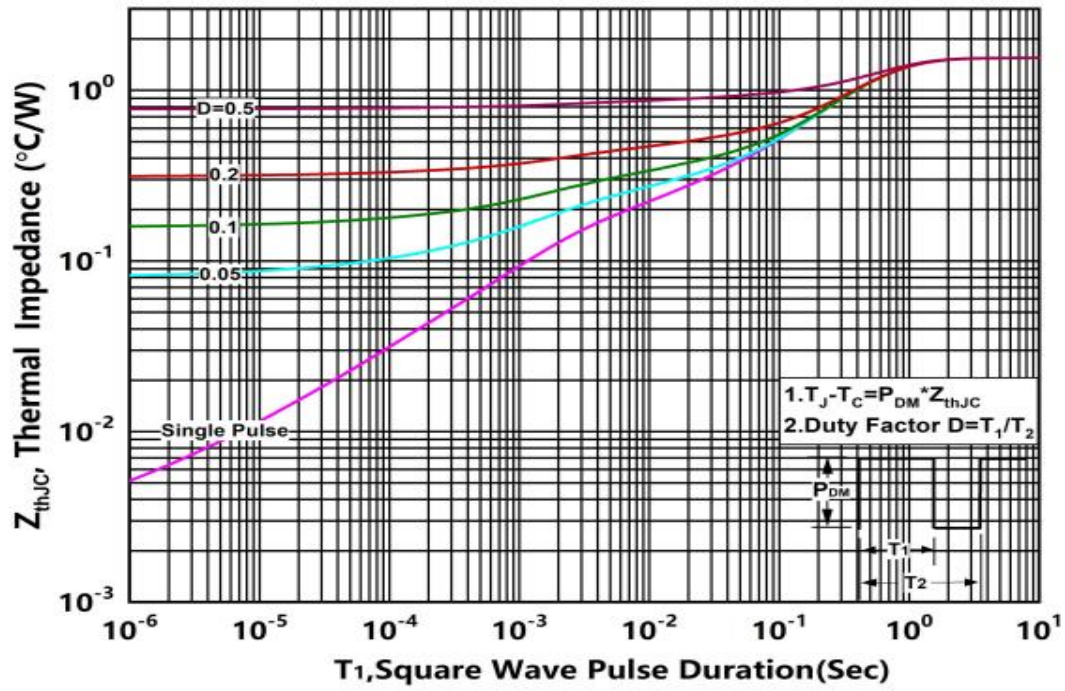
Figure.12 Transient Thermal Impedance (Junction - Case)
