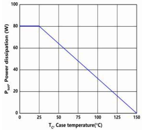
Figure.10 Maximum power Dissipation Derating vs Case Temperature
