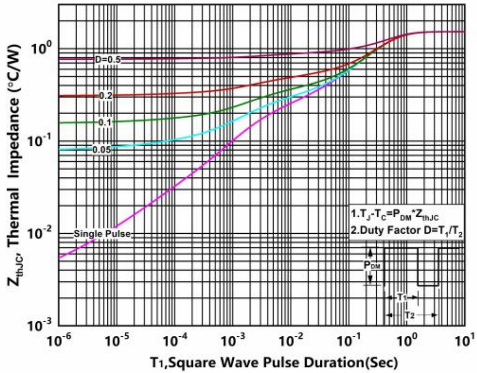
Figure.12 Transient Thermal Impedance (Junction - Case)
