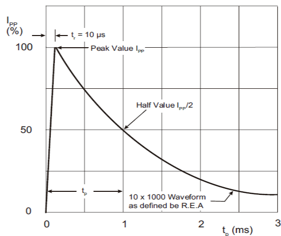
Figure2. Pulse waveform
