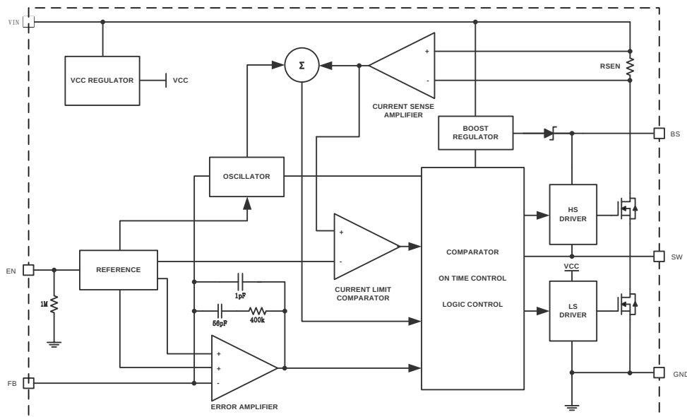
Figure 2. MSXRP7665IDBTR-F Block Diagram
