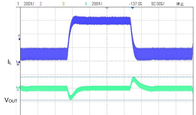
(16) Load Transient(VIN=50.0V,VOUT=12V,IOUT=0.1→0.6A)
