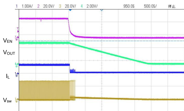
(18) Enable Shutdown(VIN=30.0V,VOUT=3.3V,IOUT=0.6A)
