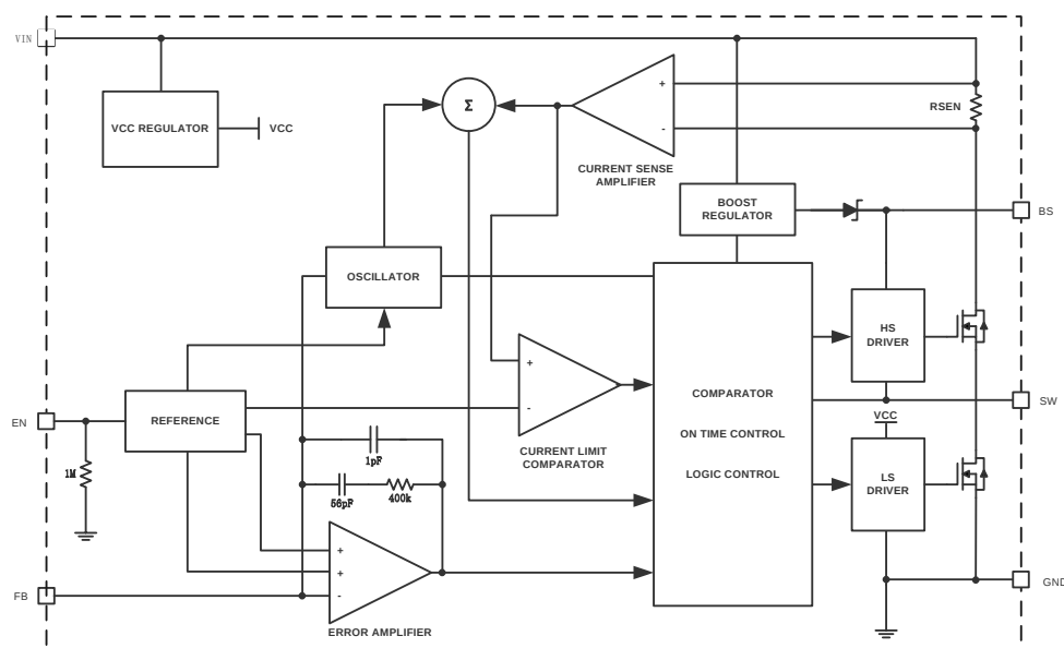
Figure 2. MSMP2303ADN-LF-Z Block Diagram
