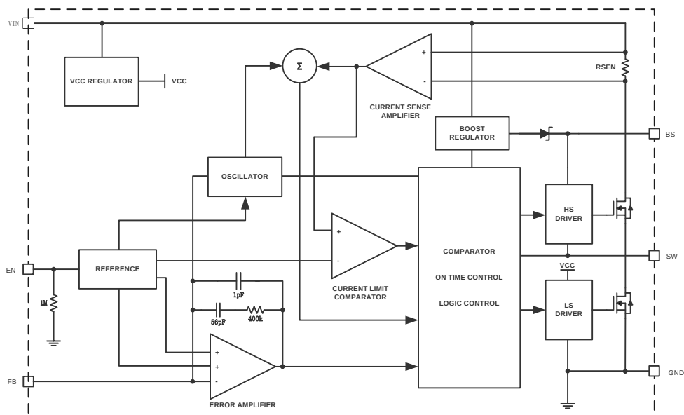
Figure 2. MSMP1482DS-LF-Z Block Diagram
