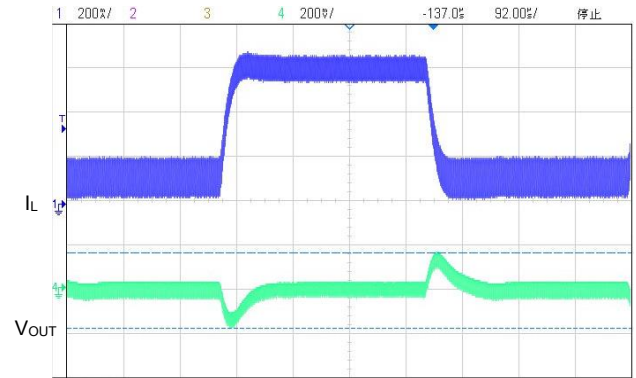
(16) Load Transient (VIN=50.0V,VOUT=12V,IOUT=0.1→0.6A)
