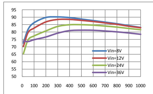
Efficient @Vout=3.3V
