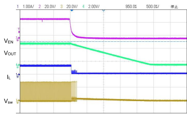
(18) Enable Shutdown(VIN=30.0V,VOUT=3.3V,IOUT=0.6A)
