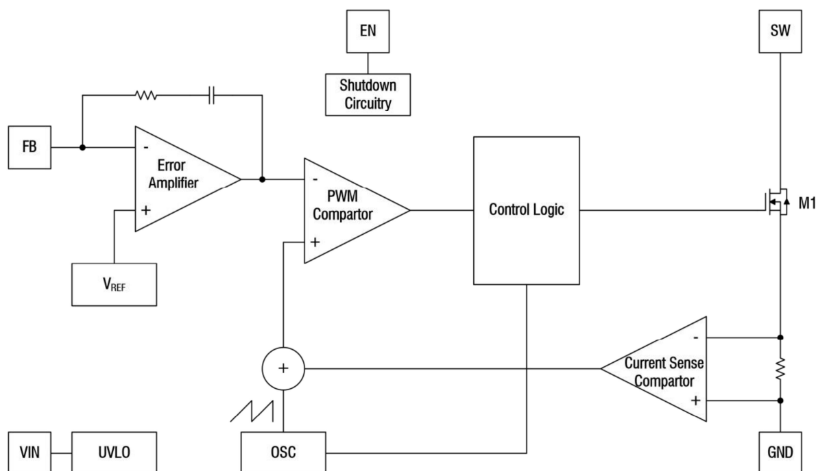
Figure 2. MSY7208ABC Block Diagram
