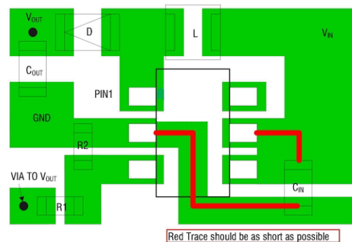
Figure 3. MSY7208ABC Suggested Layout
