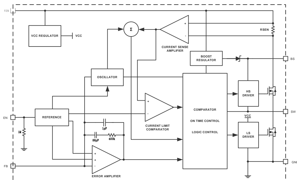
Figure 2. MSTD1484AMR Block Diagram
