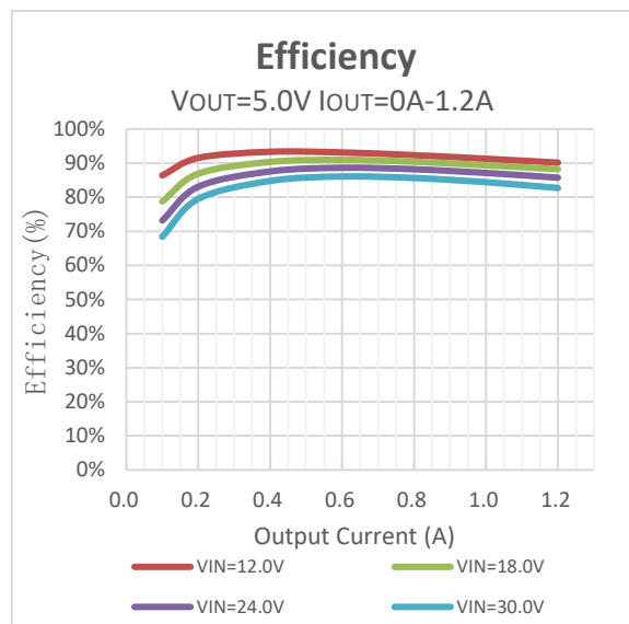
Efficiency V OUT =5V
