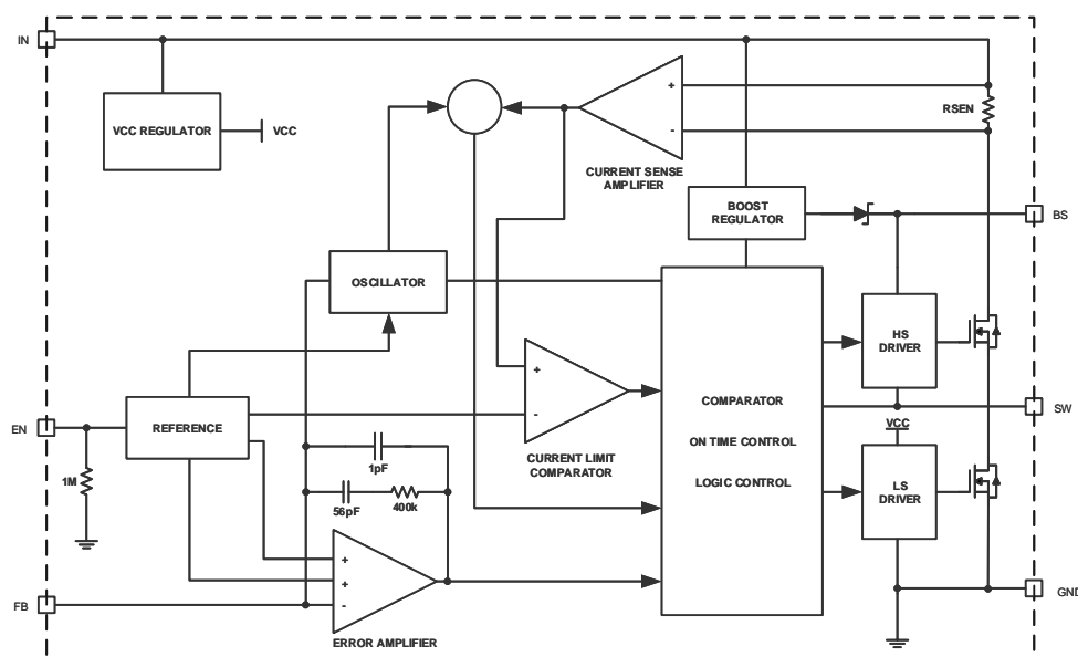
MS2359DJ-LF-Z Block Diagram
