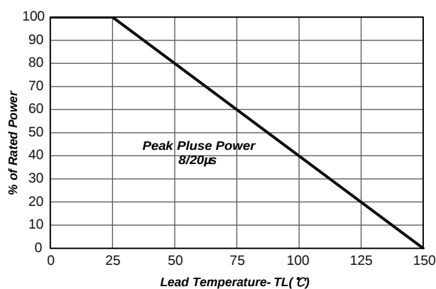
Fig2.Power Derating
