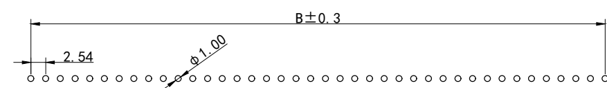
RECOMMENDED PCB LAYOUT COMPONENT SIDE VIEW
