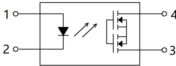
Pin Configuration
