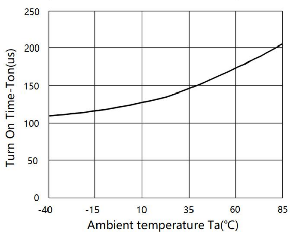
Fig.7 Turn On Time vs Ambient Temperature
