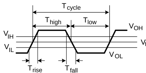
Figure 16. Output Timing
