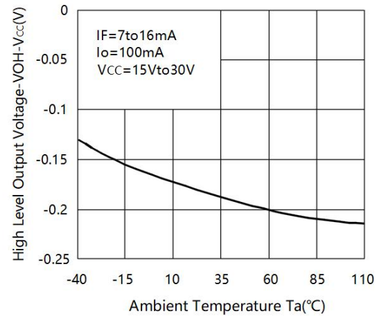
Fig.2 High Level Output Voltage vs Ambient temperature
