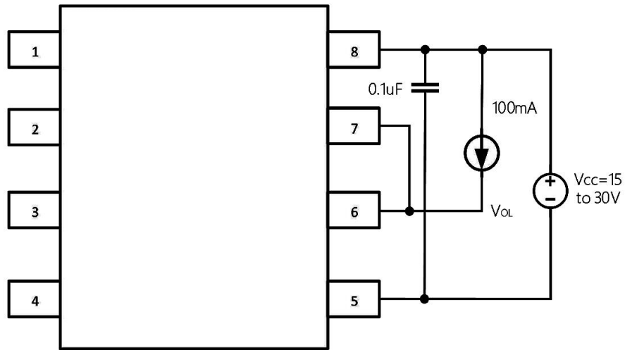
Fig.15 V OL Pulsed Test Circuit
