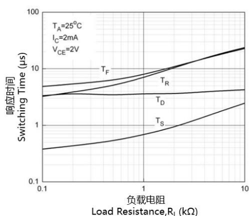
Fig.10 Switching Time vs. Load Resistance Diagram
