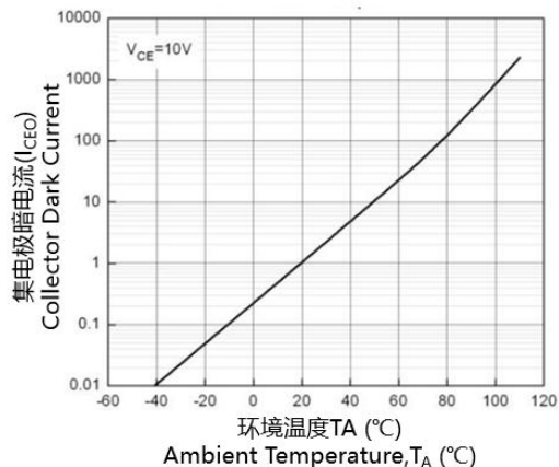
Fig.8 Collector Dark Current vs. Ambient Temperature Curve
