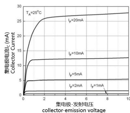
Fig.6 Collector Current vs. Collector-Emission Voltage Diagram
