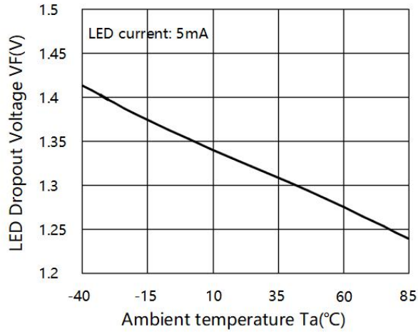
Fig.1 LED Dropout Voltage vs Ambient temperature
