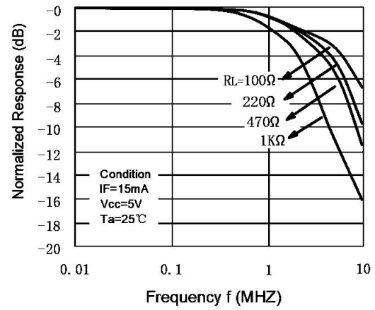
Fig.8 Frequency Response
