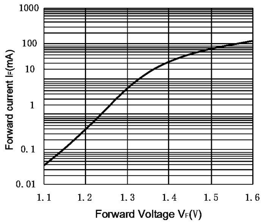
Fig.7 Forward current vs. Forward voltage
