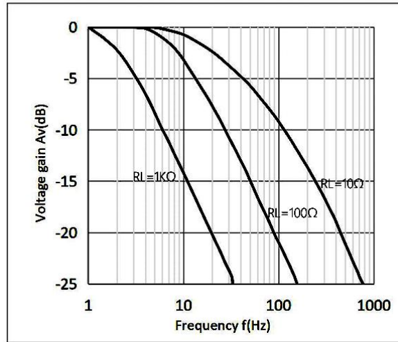
Fig.8 Frequency Response
