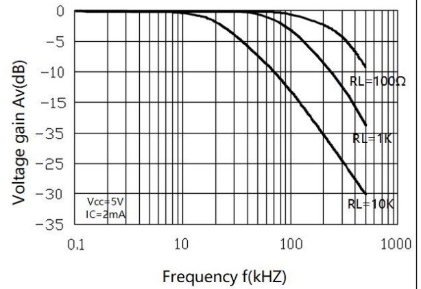
Fig.8 Frequency Response
