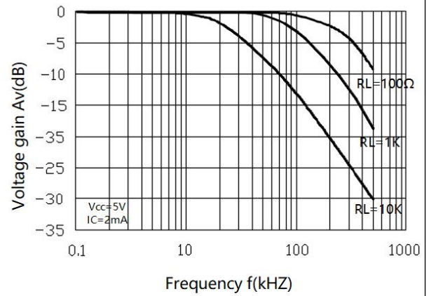
Fig.8 Frequency Response
