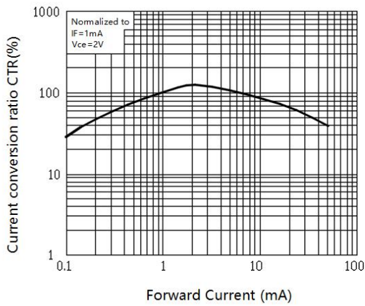
Fig1.Relative Current Transfer Ratio vs. Forward Current
