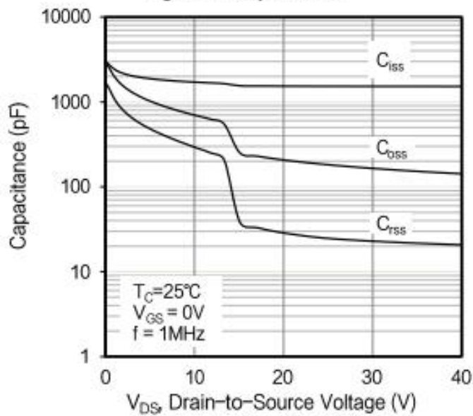
Figure 7. Capacitance
